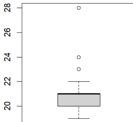
Boxplot of Age)
